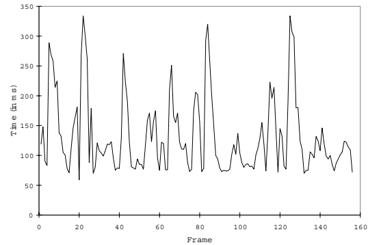
Figure 5: Plots showing (from top to bottom) instantaneous frame rates, frame rendering times (excluding optimization time) and optimization times (excluding rendering time) for each frame over the course of a typical walkthrough. The rendering cost limit is 3000, equating to 2500 single-polygon impostors. Note that the Mason-Blake algorithm is successful in ensuring constant rendering times. However the issue that is discussed in this paper is the non-constant execution of the optimization algorithm itself.
