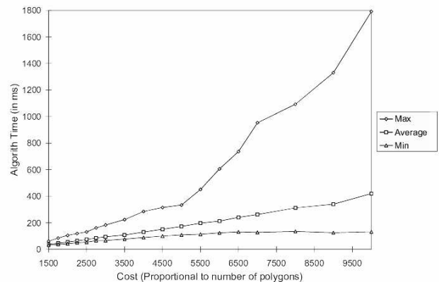
Figure 4: Plot showing how the maximum, minimum and average optimization algorithm execution times (over a typical walkthrough) vary with increasing rendering cost limit. The cost of a single polygon impostor is 1.2 units.
