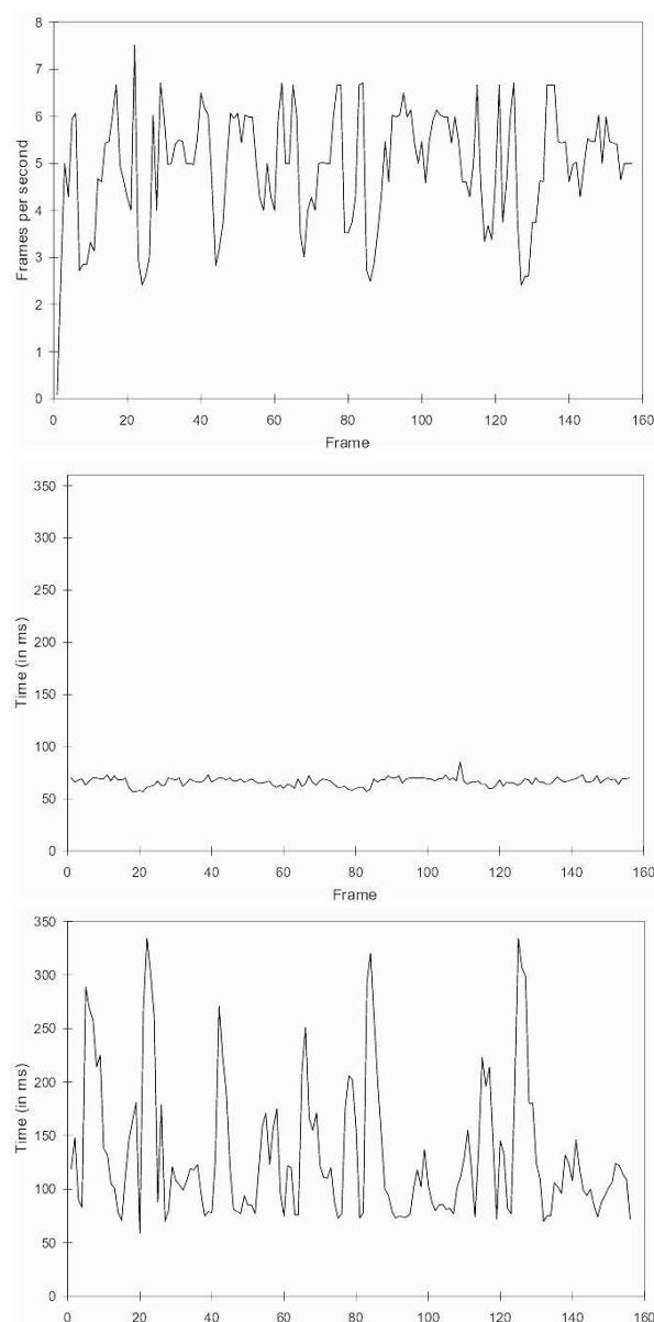
Figure 5: Plots showing (from top to bottom) instantaneous frame rates, frame rendering times (excluding optimization time) and optimization times (excluding rendering time) for each frame over the course of a typical walkthrough. The rendering cost limit is 3000, equating to 2500 single-polygon impostors. Note that the Mason-Blake algorithm is successful in ensuring constant rendering times. However the issue that is discussed in this paper is the non-constant execution of the optimization algorithm itself.
