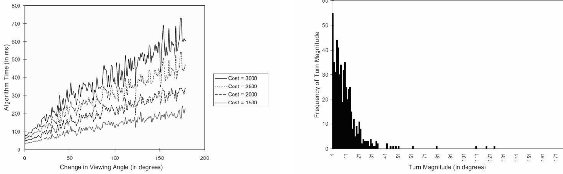
Figure 3: The figure on the left shows that the optimization algorithm execution times for various changes in viewing angle from one frame to the next along a typical path and for various rendering cost limits. The cost of a single impostor is 1.2 units. The “cost” referred to in the diagram is the rendering cost limit. Note that the change in viewing angle is usually less than 30 degrees (at 8.5 frames per second). The figure on the right shows the relative frequency of the changes in viewing angle of a typical walkthrough.
